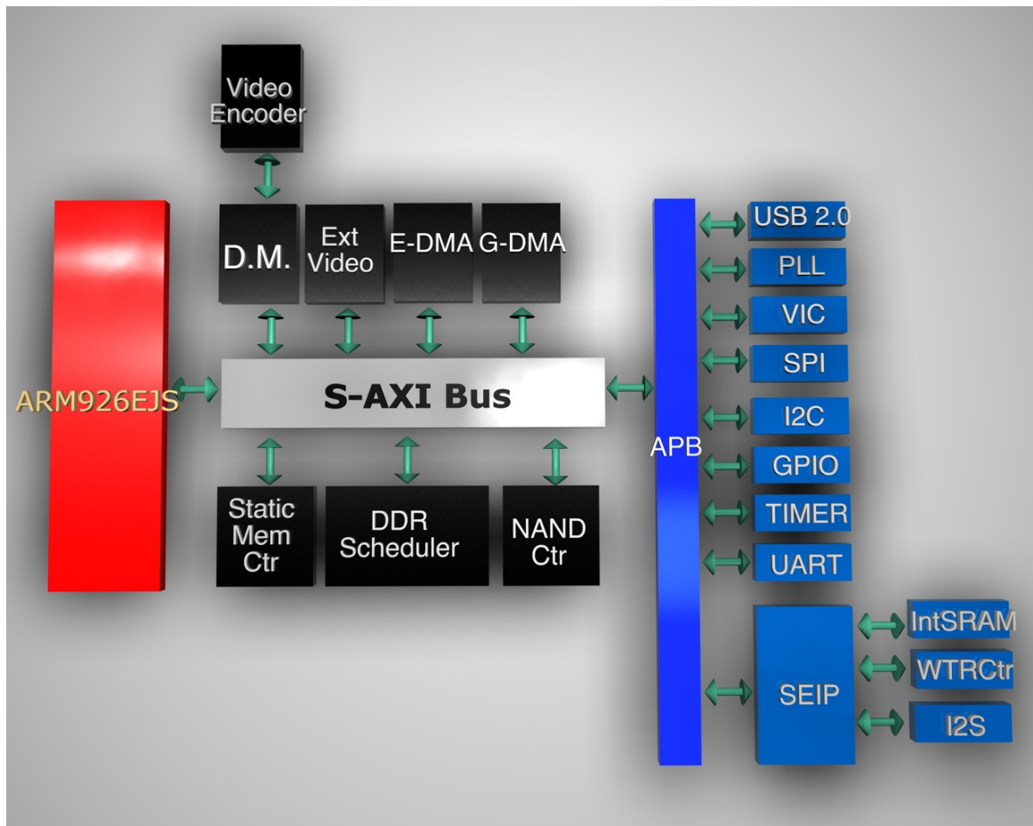
Figure 1-1 CT-500 Block diagram
