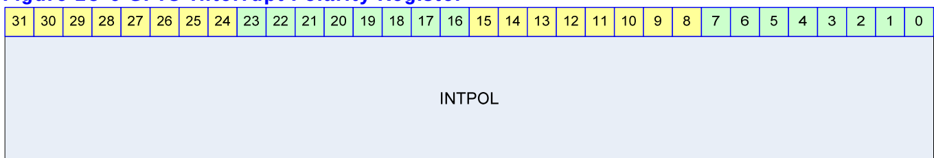
Figure 23-9 GPIO Interrupt Polarity Register
