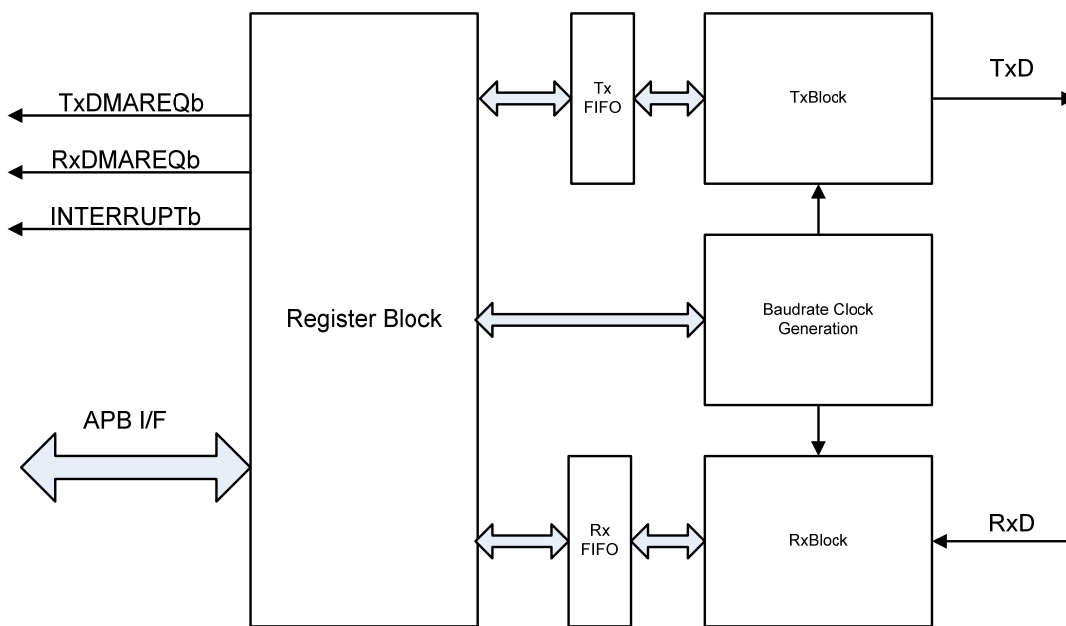
Figure 21-1 Block diagram
