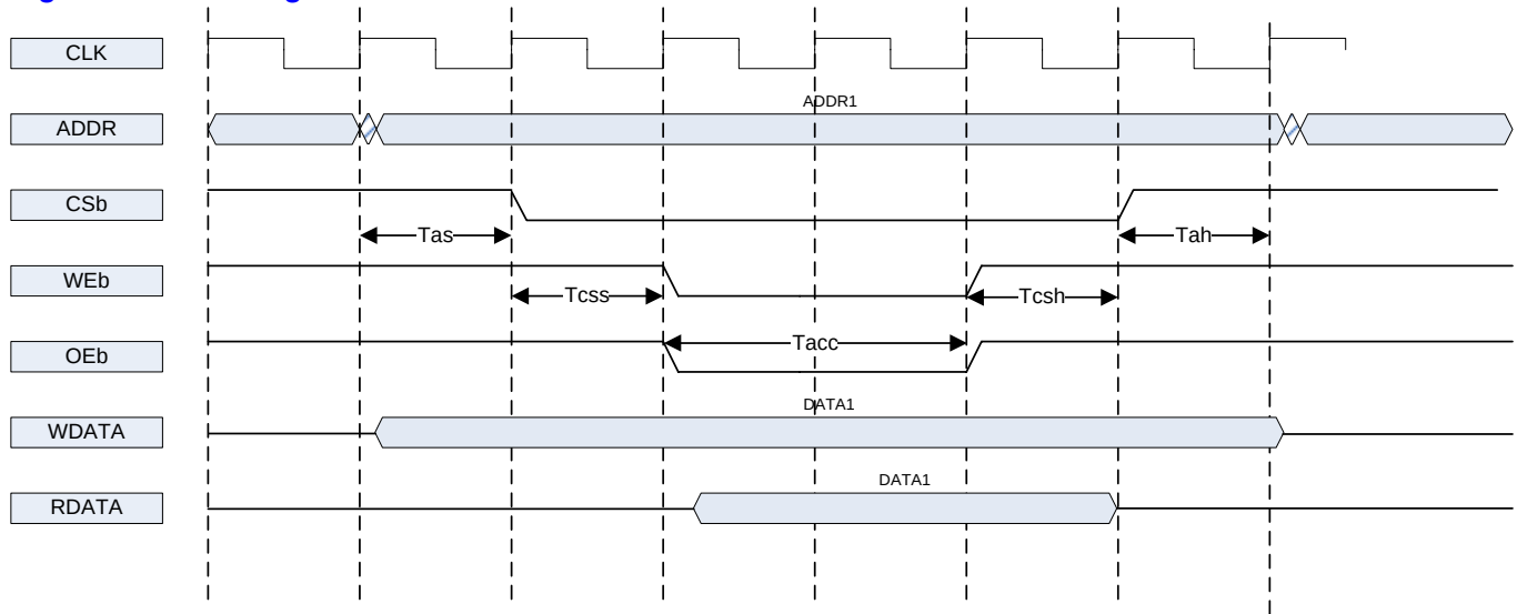
Figure 8-1 Timing
